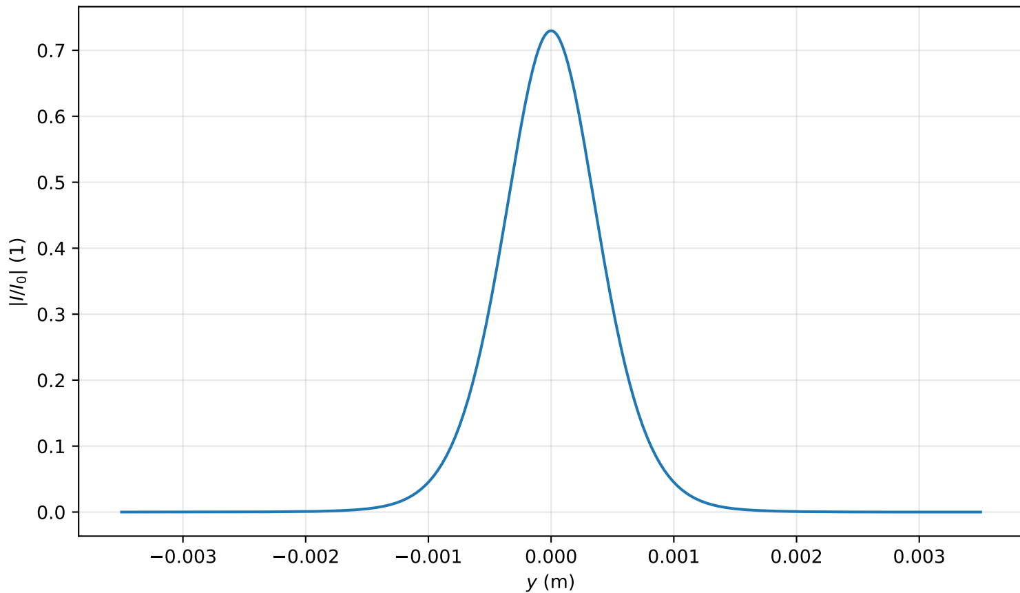
Intensity profile I(x=0, y, z=2.786)/I_0 , P_{in}=0.6P_{cr} , artificial time
